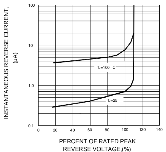
FIG.4-TYPICAL REVERSE CHARACTERISTICS
