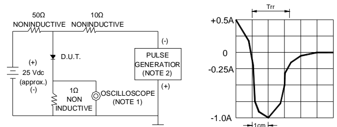
FIG.6-TEST CIRCUIT DIAGRAM AND REVERSE RECOVERY TIME CHARACTERISTIC
