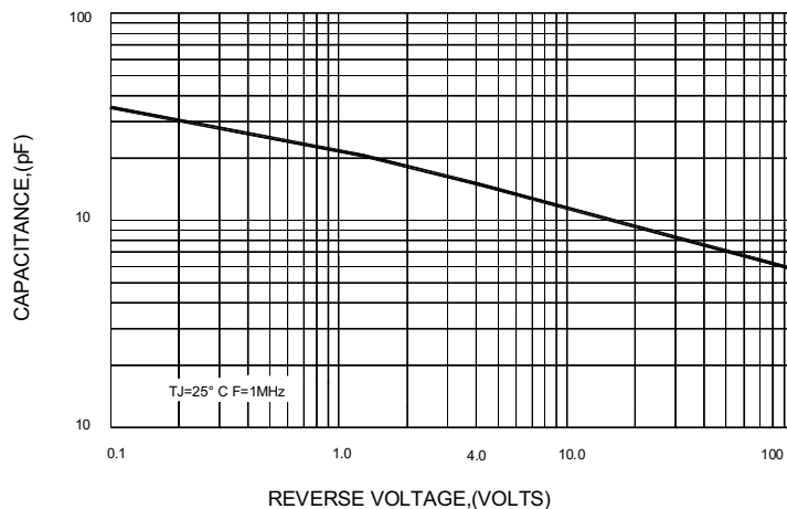
FIG.5-TYPICAL JUNCTION CAPACITANCE
